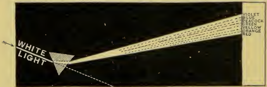
FIG. 181.—Newton's Fundamental Experiment of Decomposition of White Light by a Prism.
