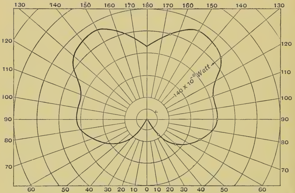
FIG. 175.—Distribution of Luminous Rays of Paraffin-Lamp (Wedding).
