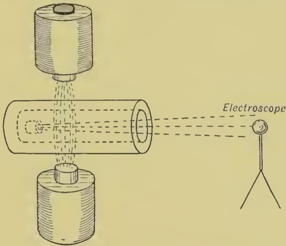
FIG. 167.—Deflexion Experiment.
