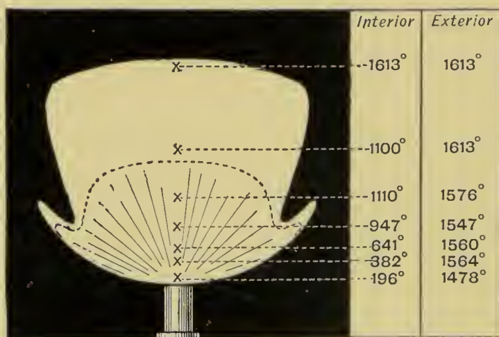
FIG. 172.—Temperatures in Gas Flame (Smithells).
