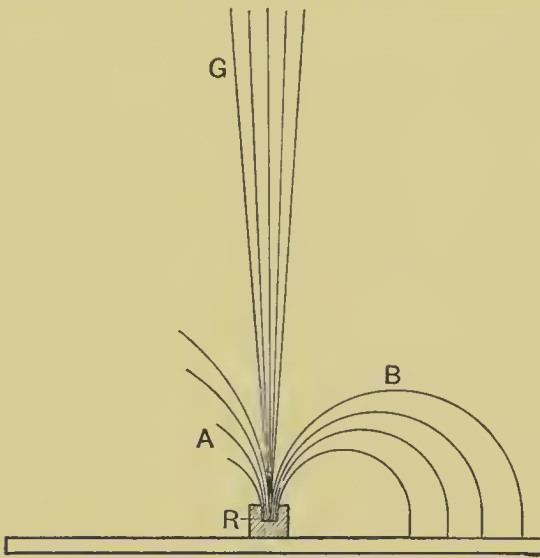
FIG. 166.—Deflexion by a Magnetic Field of the Rays emitted by Radium.
