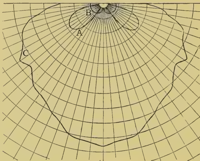
FIG. 199.—Curves of Distribution of Light of Arc-lamps.
