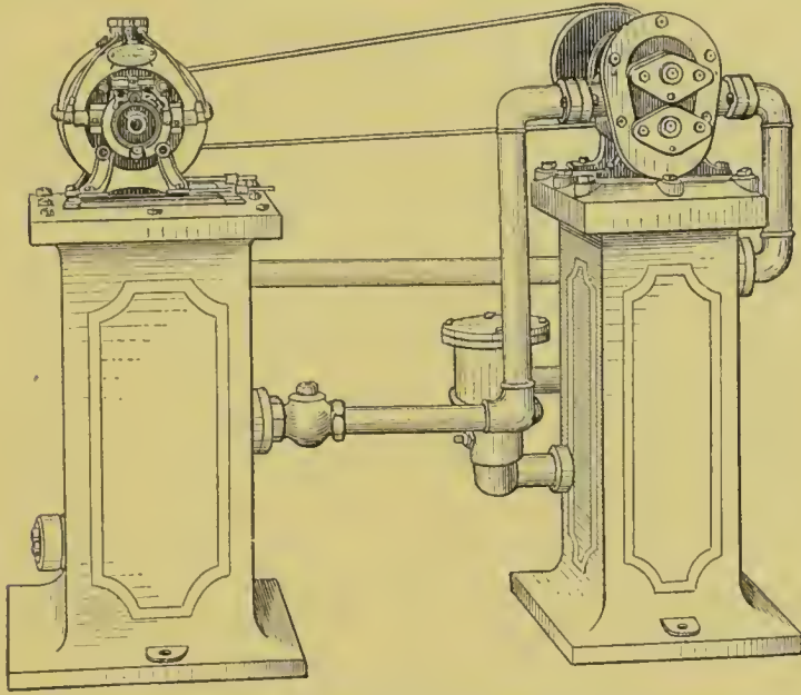
FIG. 191.—Colonia Gas Compressor for High-pressure Incandescent Gas-lighting.
