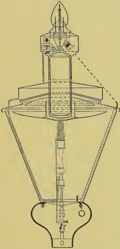
FIG. 192.—Scott-Snell self-contained High-pressure Gas Lamp.
