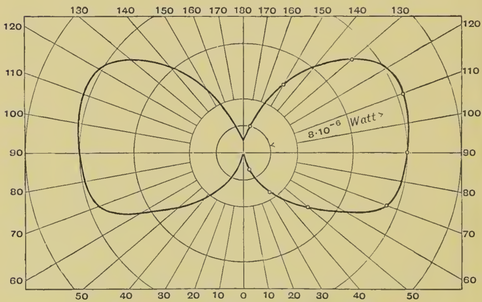
FIG. 178.—Distribution of Luminous Rays of "Millennium" Light ; High-Pressure Gas, with Long Mantle (Wedding).
