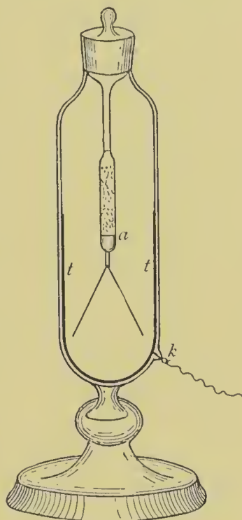
FIG. 170.—Strutt's "Radium Clock."
