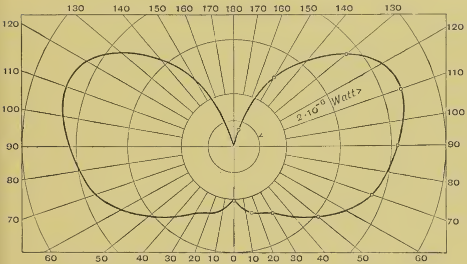
FIG. 179.—Distribution of Luminous Rays of Electric Glow-Lamp (Wedding); Watts, 59.1; Mean Spherical Candle-Power, 11.26; Watts per Candle, 5.24.
