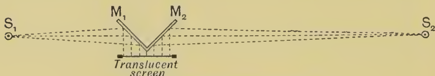
FIG. 173.—Diagram of Simple Photometer.
