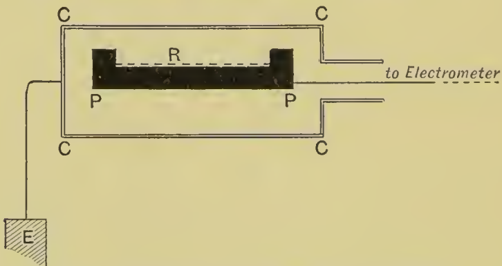
FIG. 169.—Experiment on electrification by Alpha-rays.
