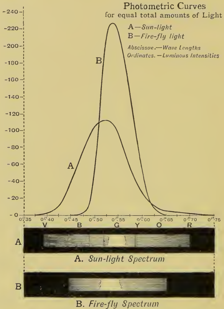
FIG. 185.—Comparative Spectra of Energy for equal amounts of Visible Radiation of Sun and Fire-fly.
