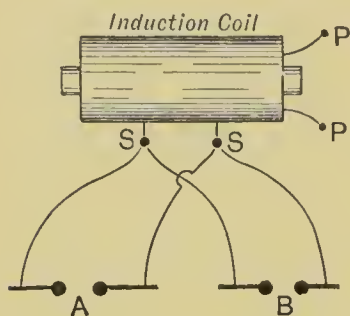
FIG. 165.—Spark-gap Experiment.
