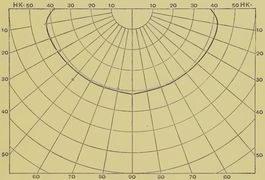
FIG. 176.—Distribution of Luminous Rays of Inverted Gas-Mantle (Wedding).
