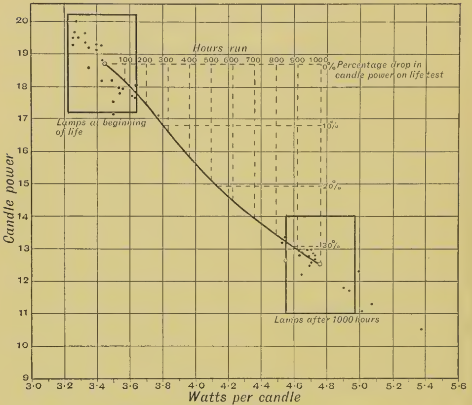
FIG. 193.—Test-chart of Twenty-four Electric Glow-lamps.
