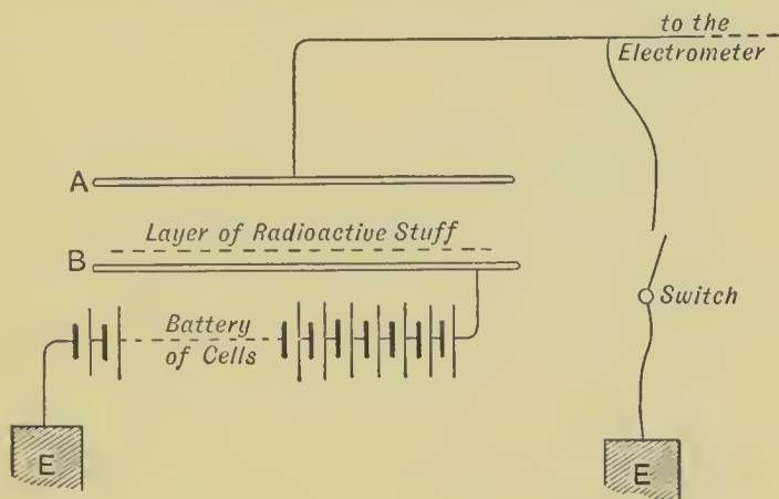
FIG. 162.—Madame Curie's Apparatus for detecting Radio-Activity.
