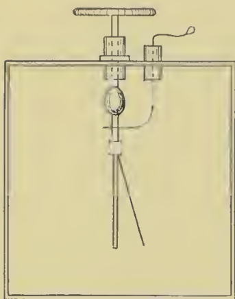
FIG. 161.—Electroscope suitable for Observation of Radio-Activity.
