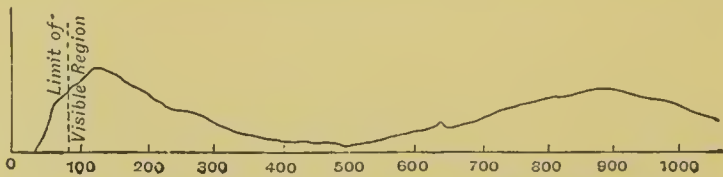
FIG. 190.—Rubens' Curve for Emissivity of Welsbach Mantle.
