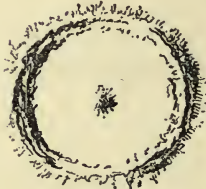
THEOPHILUS. 64 Miles Diam r
