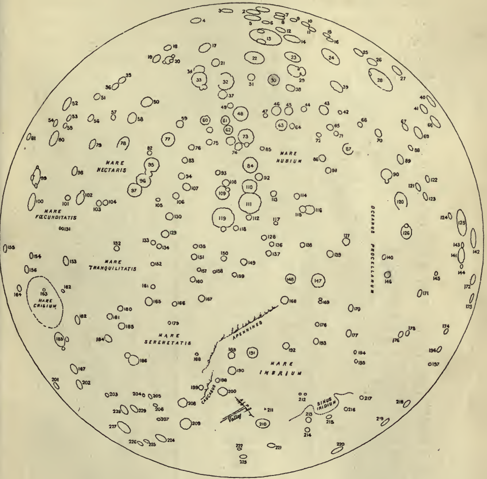
SKELETON MAP OF THE MOON. TO ACCOMPANY PICTURE MAP (Plate V.).
