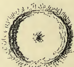
ALPHONS 70 Miles Diam r
