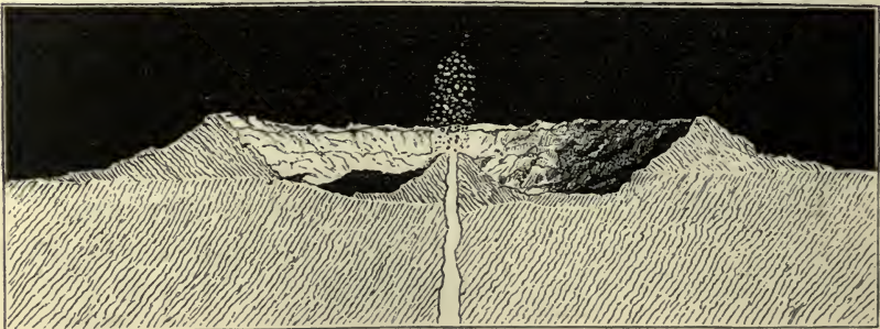
THE FORMATION OF THE CENTRAL CONE. FINAL ACTION OF A LUNAR VOLCANO.
