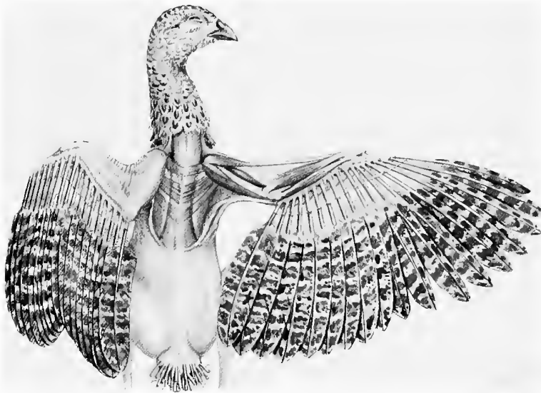
FIG. 40.—Shows the dorsal aspect of the hard and soft parts of the wing of the pheasant ( Phasianus colchicus ). In the right wing the roots of the primary and secondary feathers are exposed to show their relation to the fore arm, hand, and greatly modified phalanges or finger bones. The left wing is fully flexed and ready to make the up stroke. In the left wing the feathers are widely separated, and present a series of vertical knife-like edges through which the air escapes during the up stroke; in the right wing the feathers are spread out and firmly pressed together to prevent the escape of air during the down stroke. (From a dissection and drawing by the Author.)
