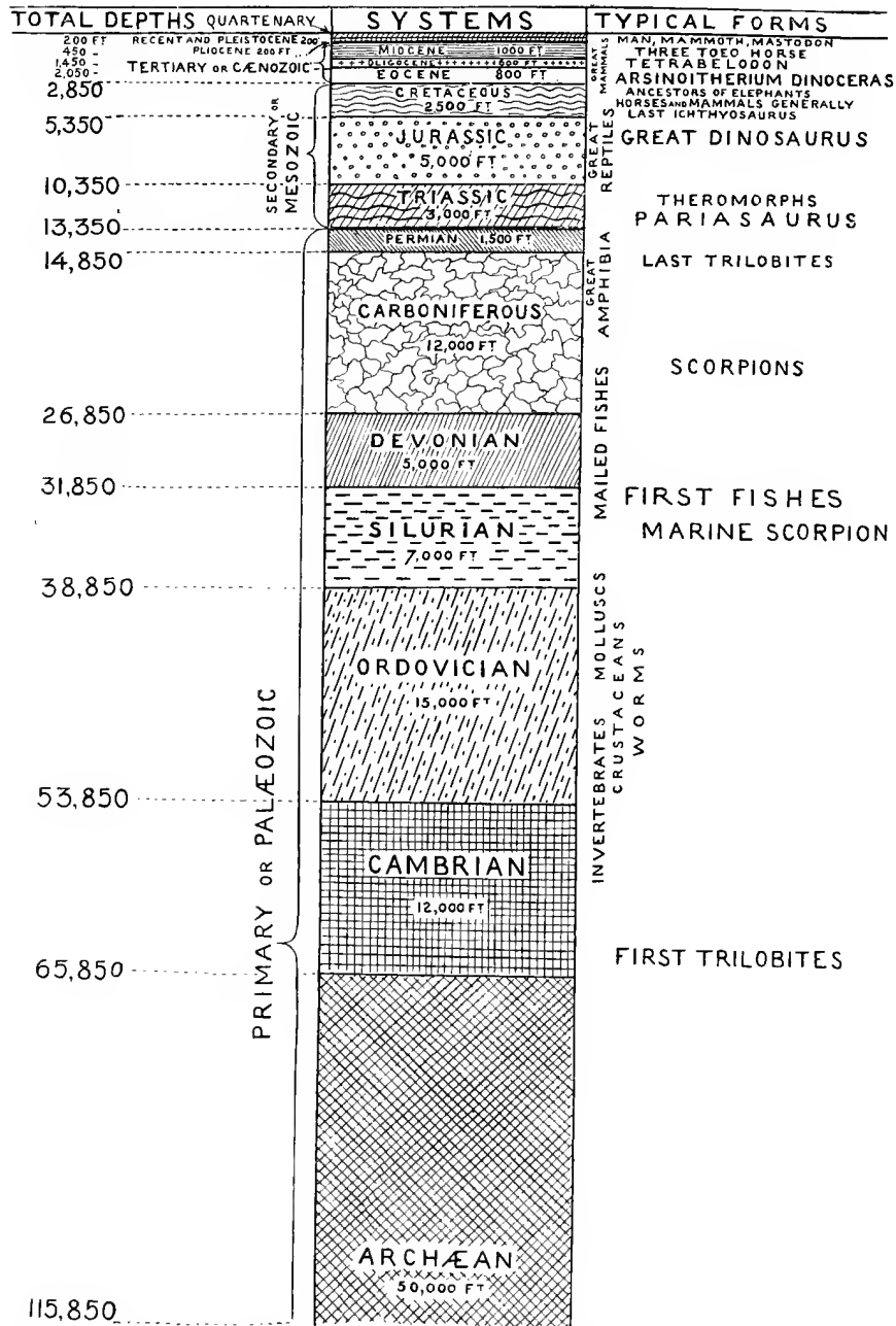
FIG. 44.—A tabular view of the strata of the earth's crust, showing the relative thickness of each "system" or group of strata, and the position in which important animal remains have been discovered. The rocks are never found lying horizontally. In nature they are tilted and crumpled, but we can make out their thickness and the order in which they lie one over the other (after Lankester).
