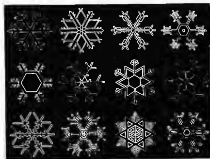
FIG. 1.—Exquisite crystals of snow as figured by Scoresby. Illustrate straight-line formations.
