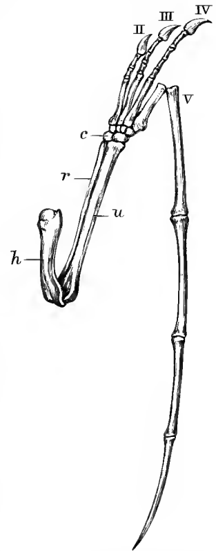
FIG. 37.—Bones of the wing of the Pterodactyl ( Scaphognathus crasirostris ) or flying reptile. Shows that the second, third, and fourth digits of the hand are aborted and terminate in claws, and that the fifth digit is thickened and enormously elongated for the purpose of supporting and carrying the flying membrane which constitutes the essential part of the wing as far as flight is concerned (after Nicholson and Lydeker).
