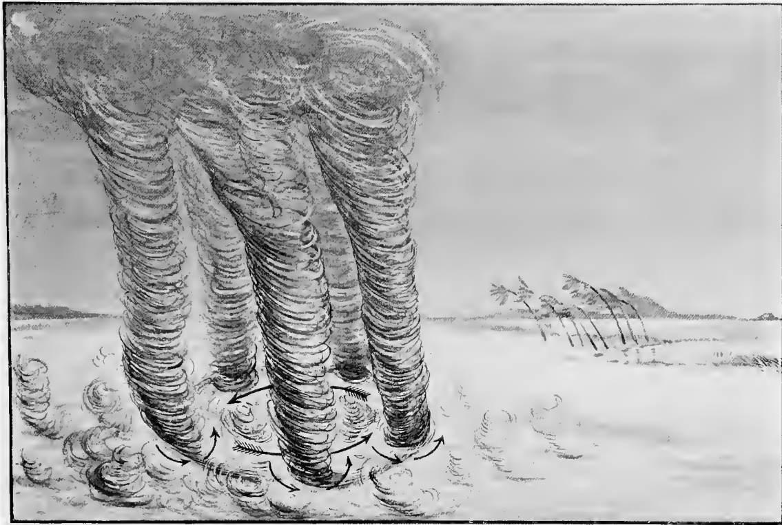
FIG. 3.—Study of a spiral sand-storm by the Author. Drawn by C. Berjeau.
