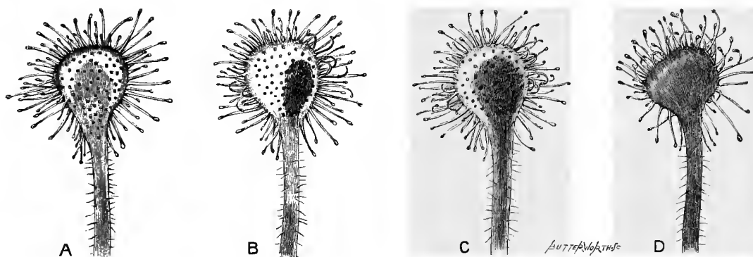
FIG. 30.—Shows the clouding or staining of the leaf of the sundew during digestion (magnified twice).
