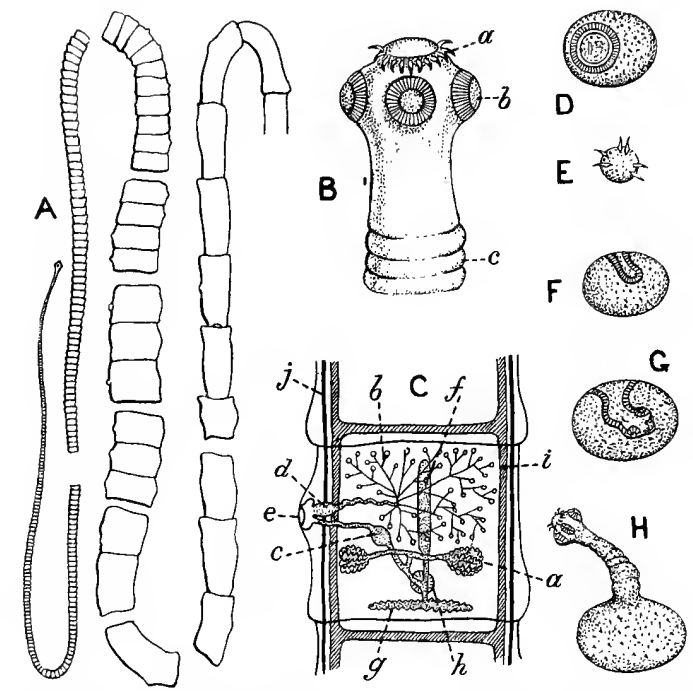
FIG. 34.—A. Tænia saginata . B. Head of Tænia solium . C. Semi-diagrammatic view of a single proglottis of tænia . a, Ovary; b, testis; c, receptacle; d, seminal vesicle; e, common sexual aperture; f, uterus; g, yolk-gland; h, shell-gland; i, excretory canal; j, nerve cord. D, E, F, G, H. Development of Tænia solium (after Leuckart).
