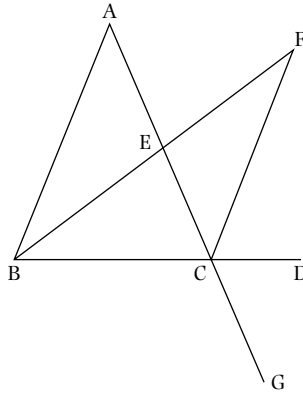
Fig. 11 The picture for Euclid I.16.
