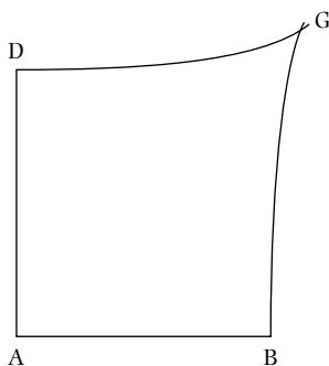
Fig. 8 Lambert's quadrilateral.
