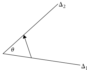
Fig. 1 The 'half-line angle' (\widehat{\Delta_1, \Delta_2}) is the angle of rotation from the first line to the second.
