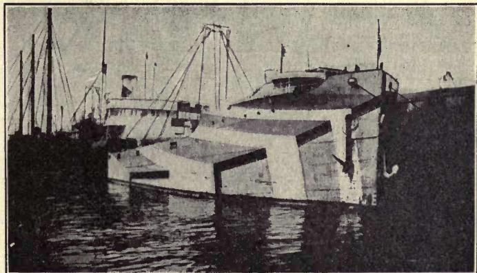
Figs. 97 and 98. — Examples of the geometrical-optical illusion as finally applied.
