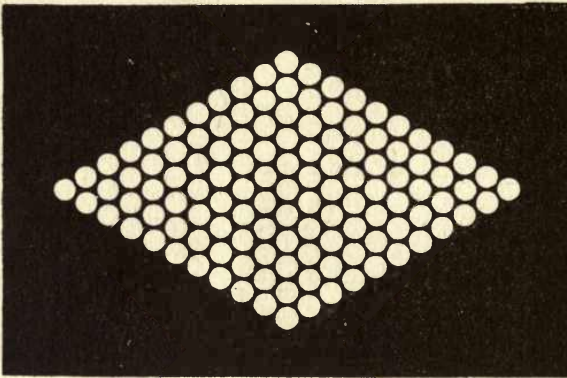
Fig. 28. — The grouping of the circles fluctuates.
